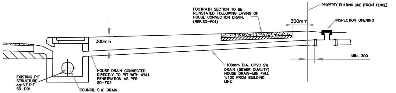
HOUSE DRAIN - DIRECT DRAIN CONNECTION
