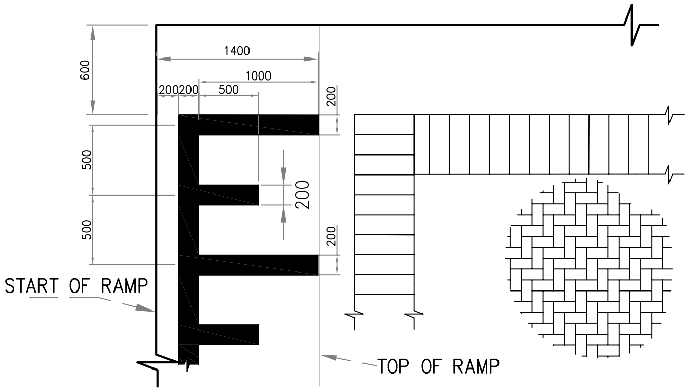
TYPE 'A' RAMP: HIGH VOLUME TRAFFIC
