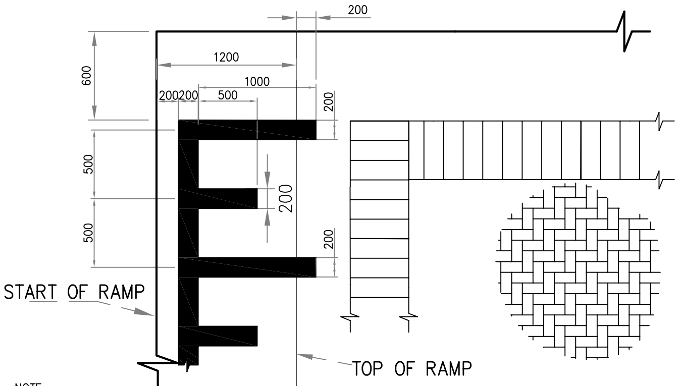
TYPE 'B' RAMP: LOW VOLUME TRAFFIC
