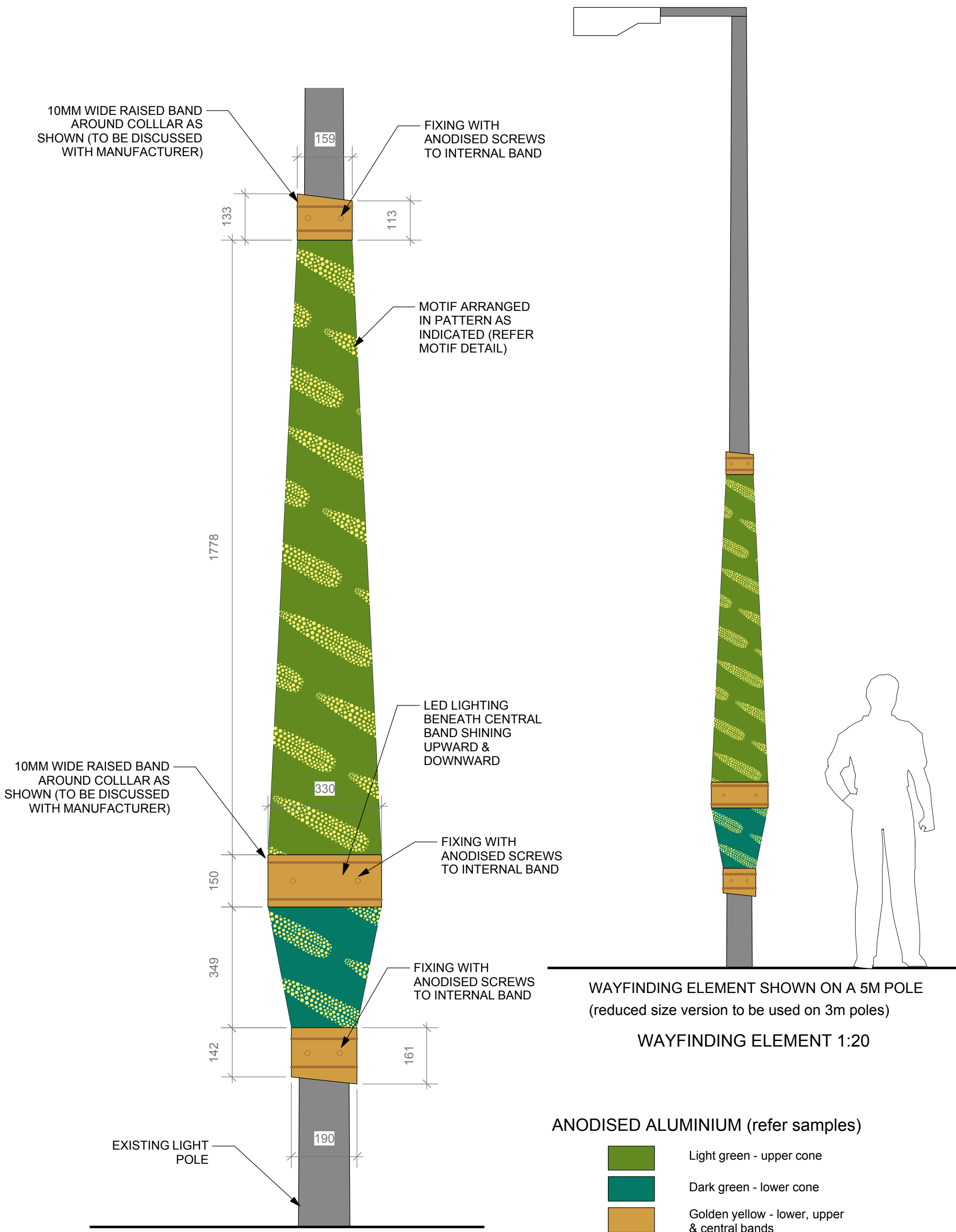
WAYFINDING ELEMENT 1:10
