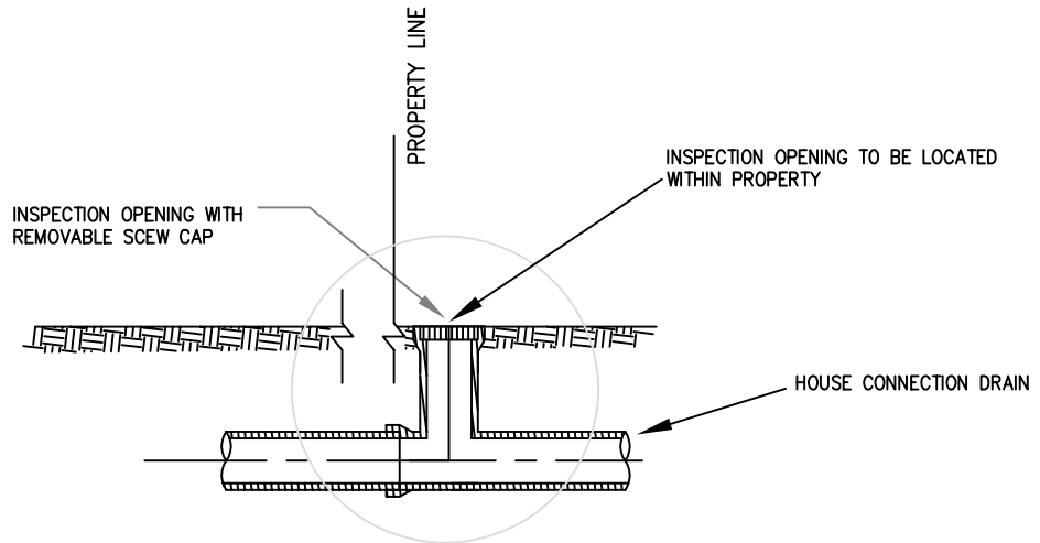
TEE PIECE INSPECTION OPENING
