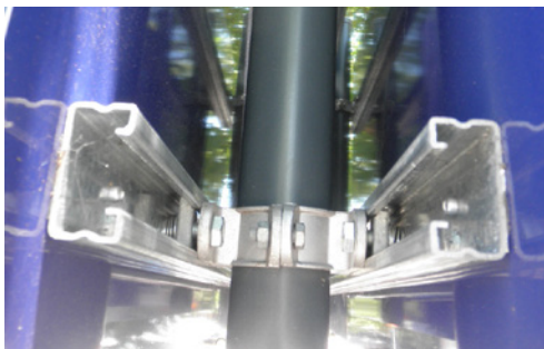
Double-sided Installation with spring nuts
