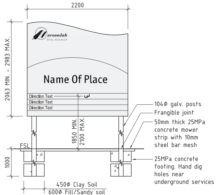
Large Sign Installation Detail - Section 1:50
