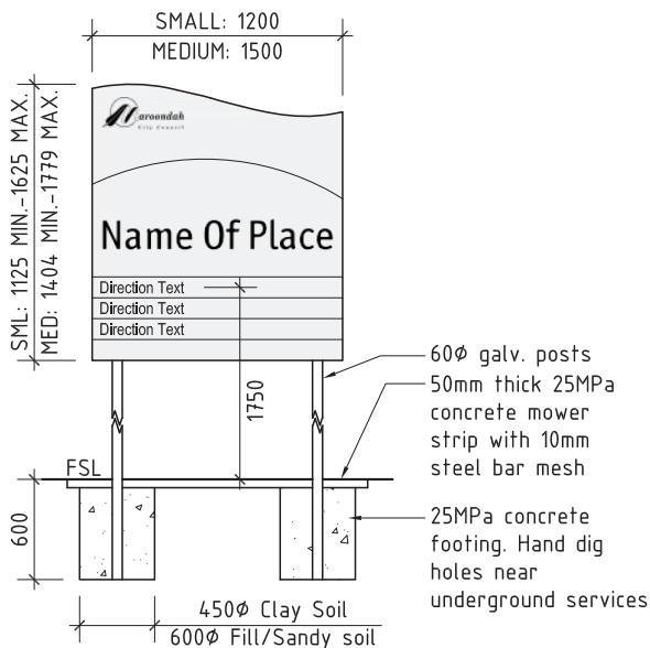
Small & Medium Sign Installation Detail - Section 1:50
