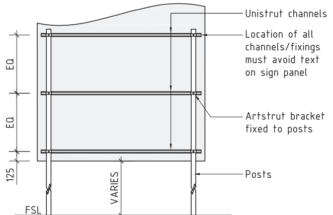
Sign Installation Detail (All Sizes) Rear Elevation Not To Scale
