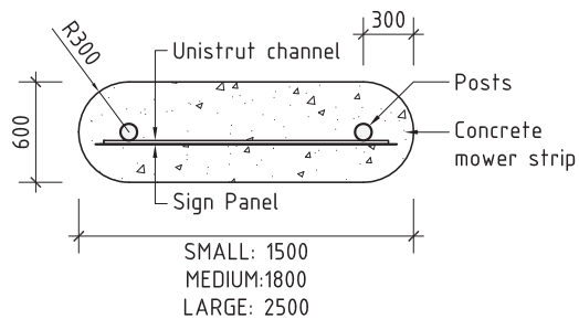
Mower Strip Detail - Plan 1:50
