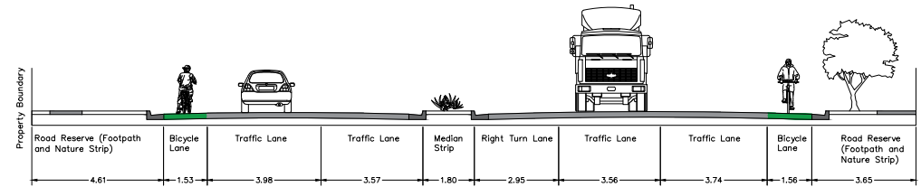
Section B-B
