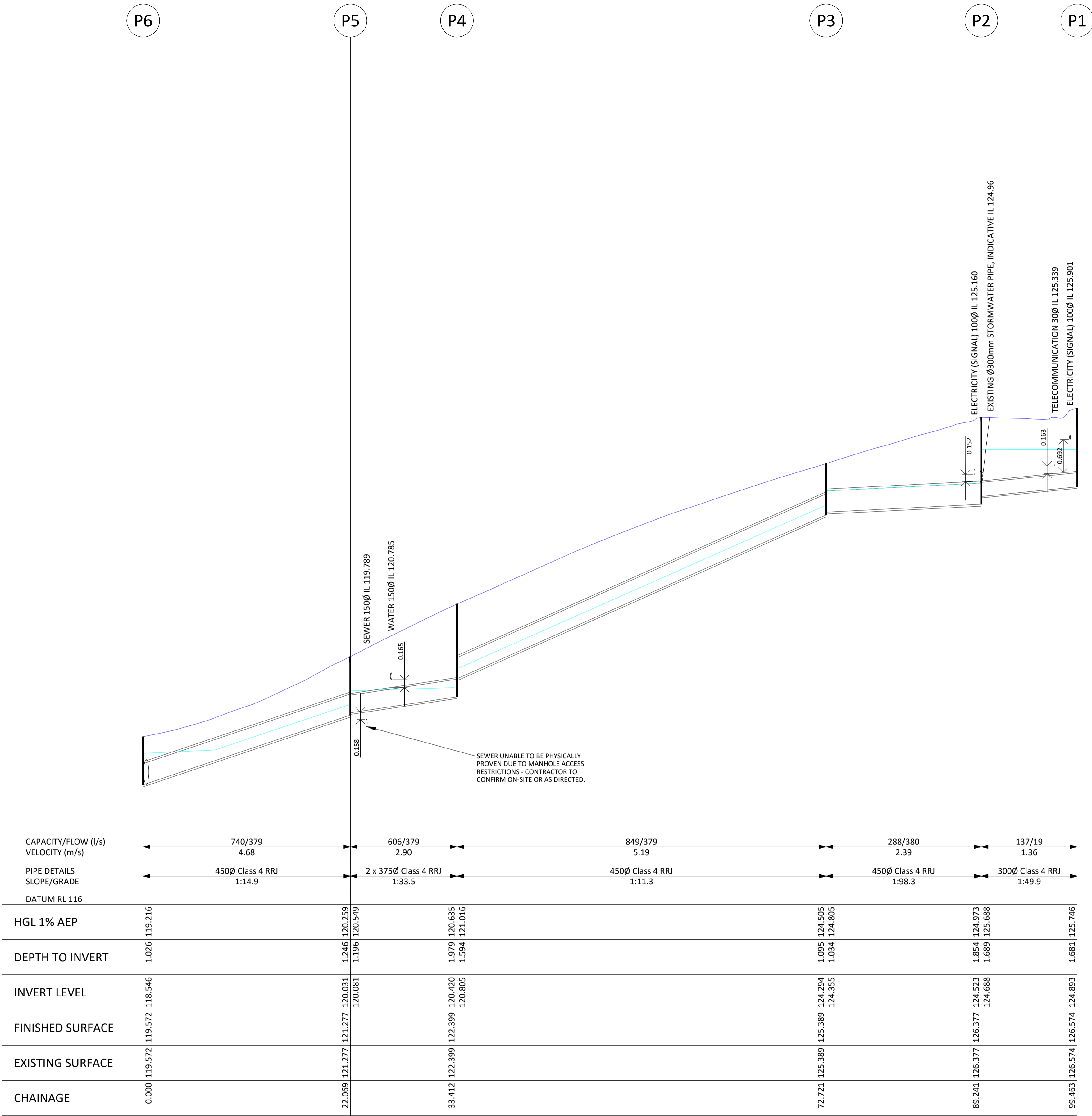
DRAINAGE LONGITUDINAL SECTION SCALES: HORIZONTAL 1:250 VERTICAL 1:50
